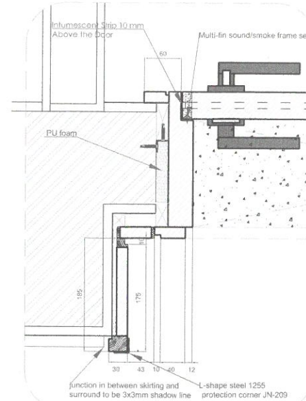
D3 Typical Frame detail
