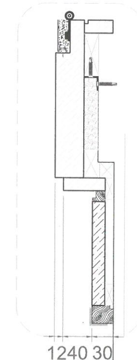
Type A and A mir. architrave
