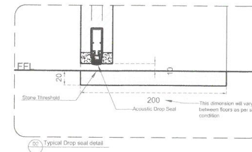
D2 Typical Drop seal detail
